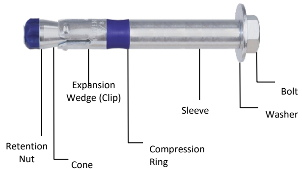
FIGURE 2—POWER BOLT+ ANCHOR ASSEMBLY
